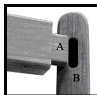
SEAT INSERTS
